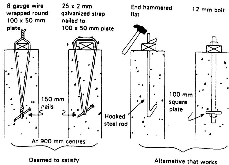
Figure 5.8: Fixings
