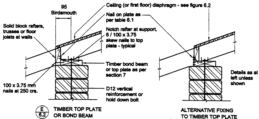
Figure 5.9: Timber bond beam-roof connection
