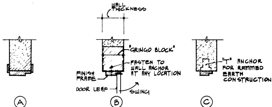
Figure 5.6: Details of door jamb sections (Reproduced from McHenry, 'Adobe and rammed earth buildings')
